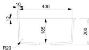
Side cross-section
