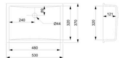
Side cross-section
