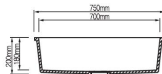
Side cross-section
