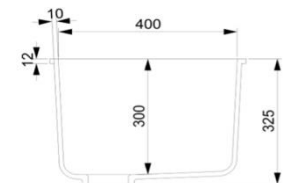
Side cross-section
