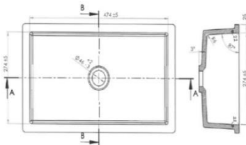
Side cross-section
