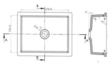
Side cross-section
